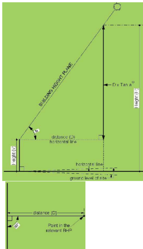
Figure 2(fg): Building Height Plane Diagrams
