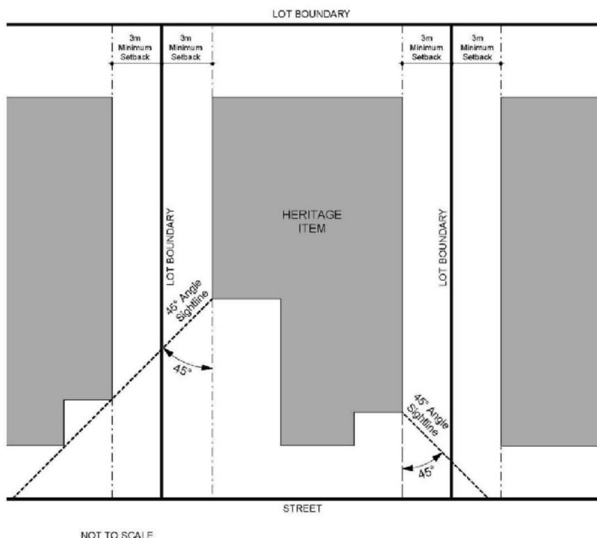
Figure 223: Minimum Setbacks for Development Adjacent to a Heritage Item or Heritage Conservation Area
