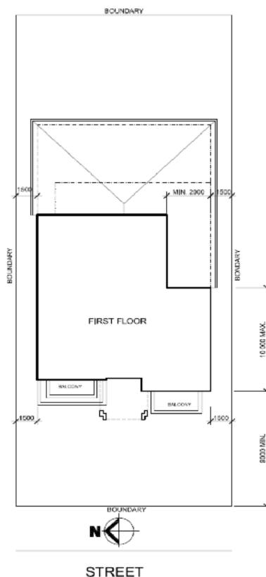
Figure 3644: Setbacks to Minimise Overshadowing
