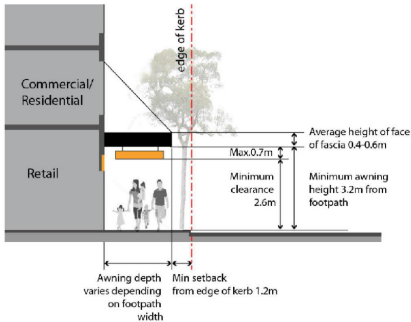
Figure 1(ei): Awning Dimensions
