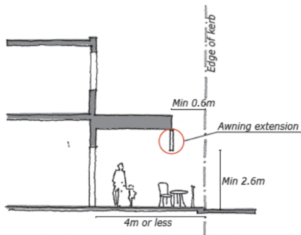
Figure 1(ek): Straight Drop Awning Extensions
