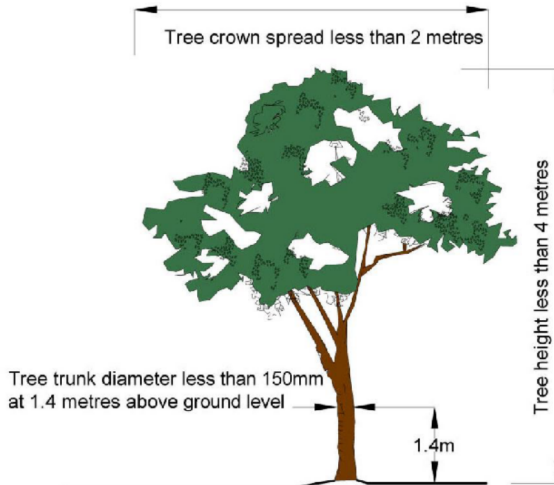
Figure 4050: Tree Dimensions for Allowable Tree Activities
