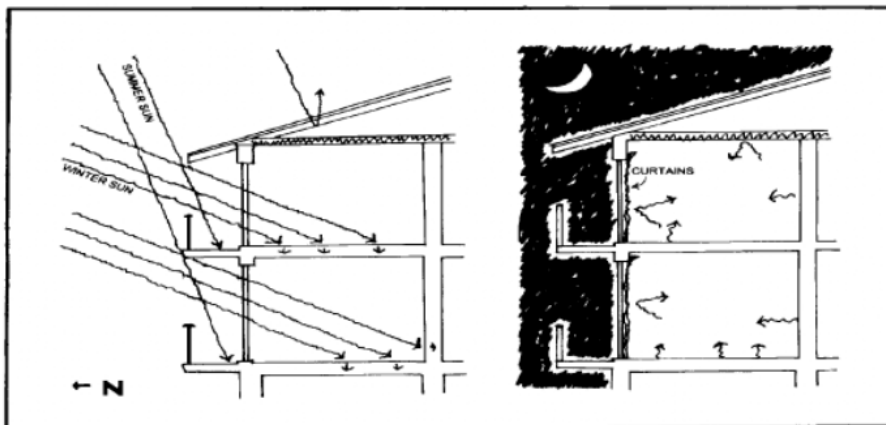
Figure 305: Solar Access and Insulation
