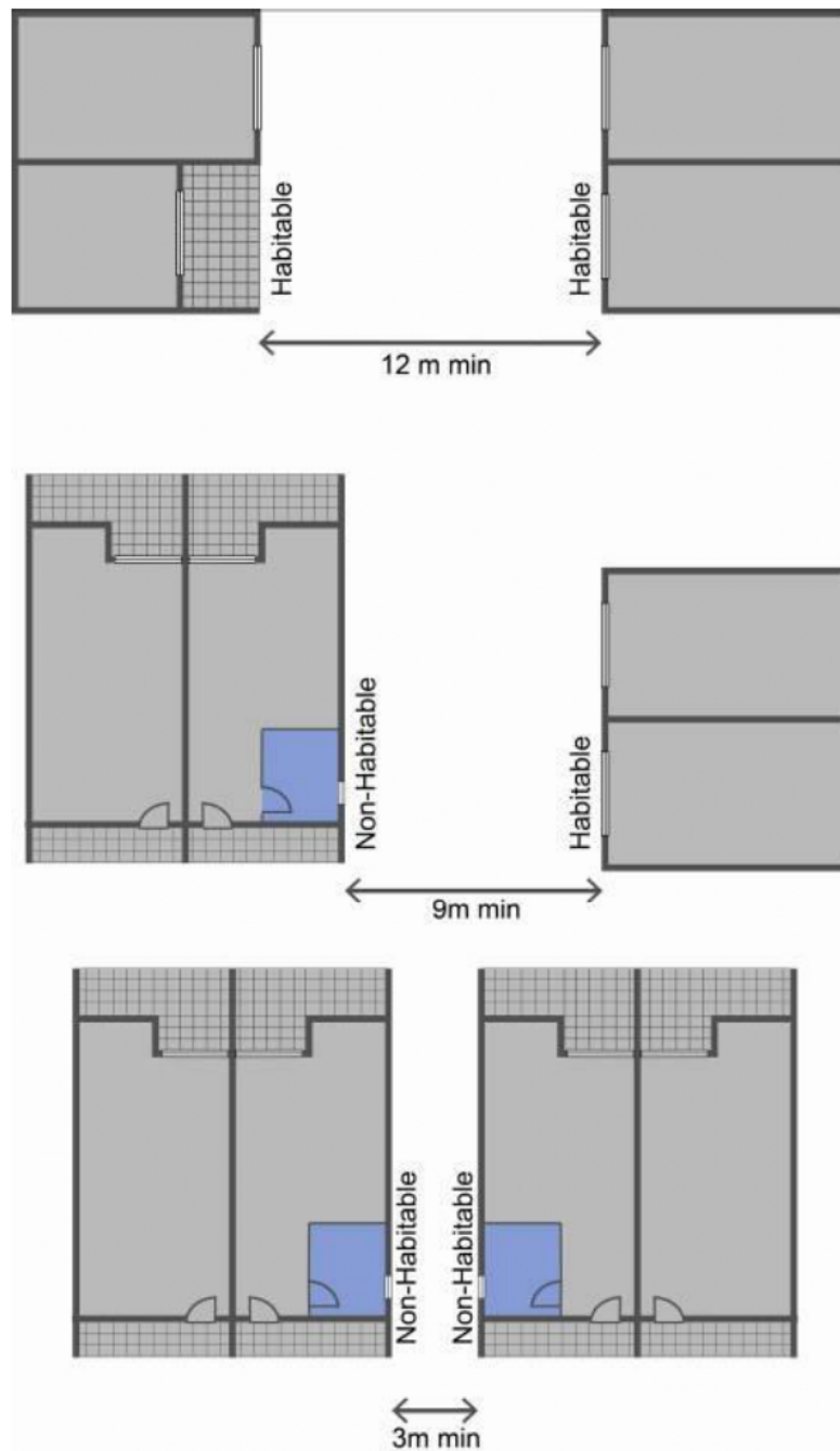
Figure 338 Building Separation for Multi Dwelling Housing
