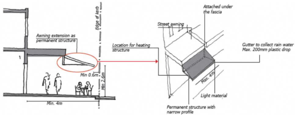
Figure 1(gm): Permanent Awning Extensions
