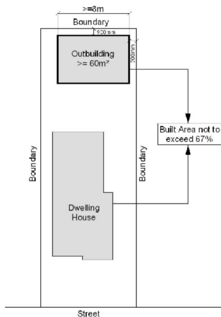
Figure 36(a)45: Boundary Setbacks for Substantial Outbuildings
