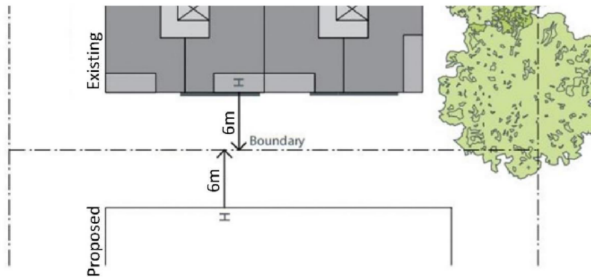
Figure 22(a) Separation distances
