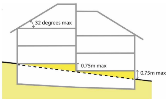
Figure 35(a) 41: Maximum Projection for Basement Car Parks on Sloping Sites and Maximum Roof Pitch
