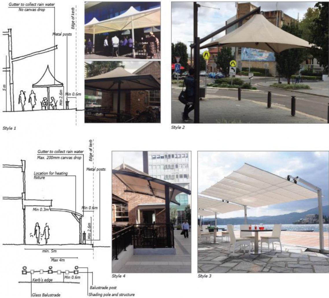
Figure 1(hn): Styles of Permanent Free Standing Awnings/Shade Structures
