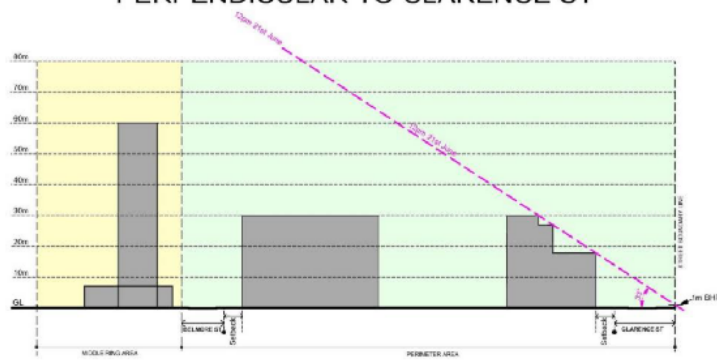
SOUTHERN BUILDING HEIGHT PLANE - 12 NOON at 33° SECTION C:C
