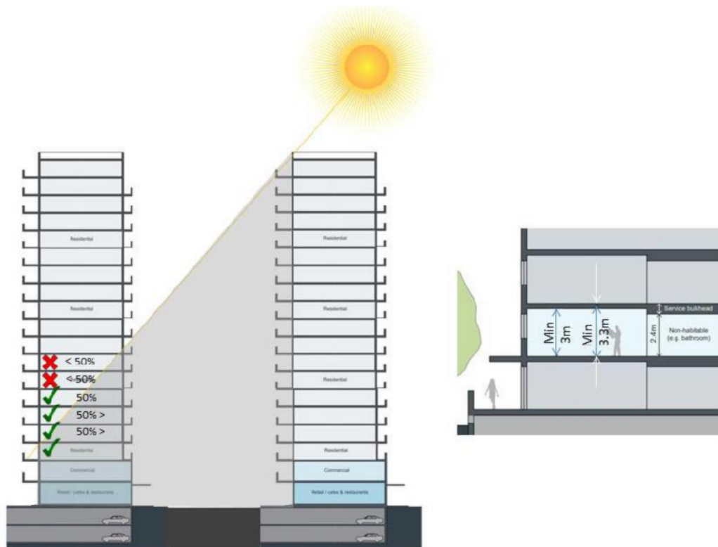
Figure 1(e). Increased floor to ceiling heights (Adapted from ADG 2015)
