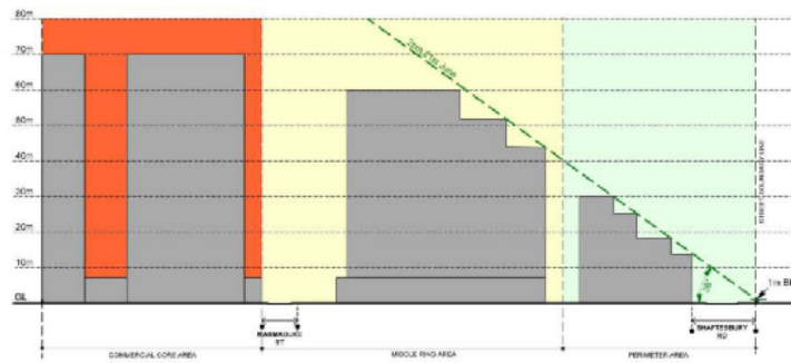
EASTERN BUILDING HEIGHT PLANE - 2 pm at 36° SECTION D:D
