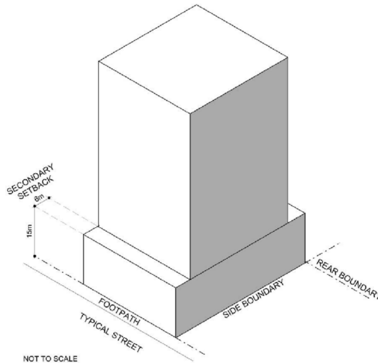
Figure 7: Commercial Core and Middle Ring Area: Typical Midblock Development Setbacks
