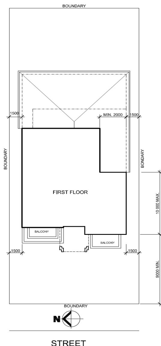
Figure 42: Setbacks to Minimise Overshadowing
