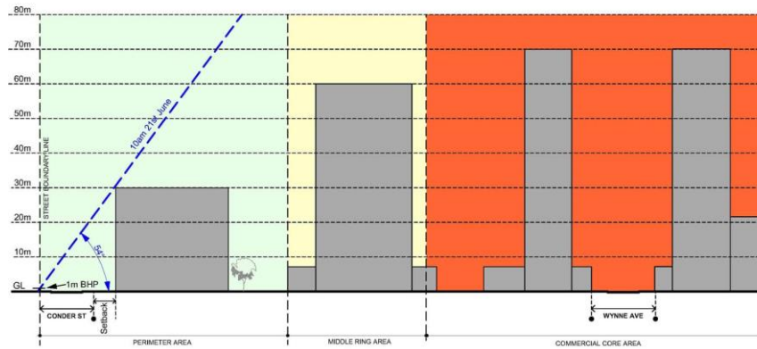
WESTERN BUILDING HEIGHT PLANE - 10am at 54° SECTION A:A
