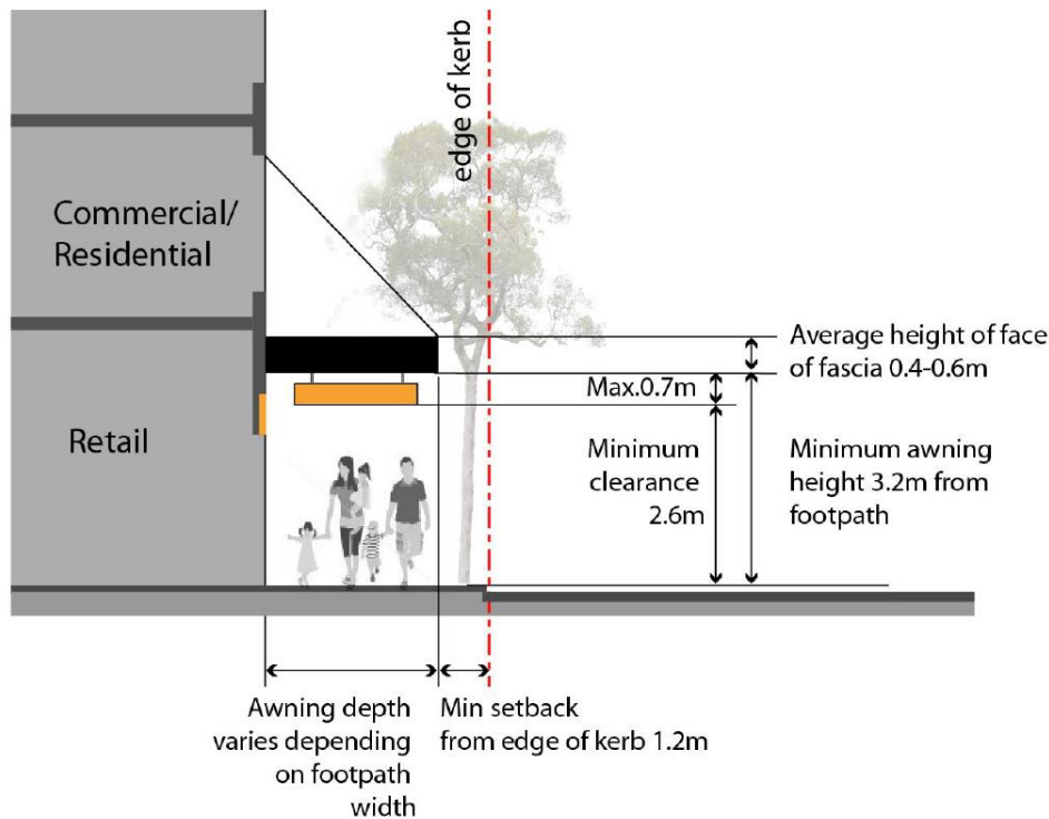
Figure 9. Awning Dimensions
