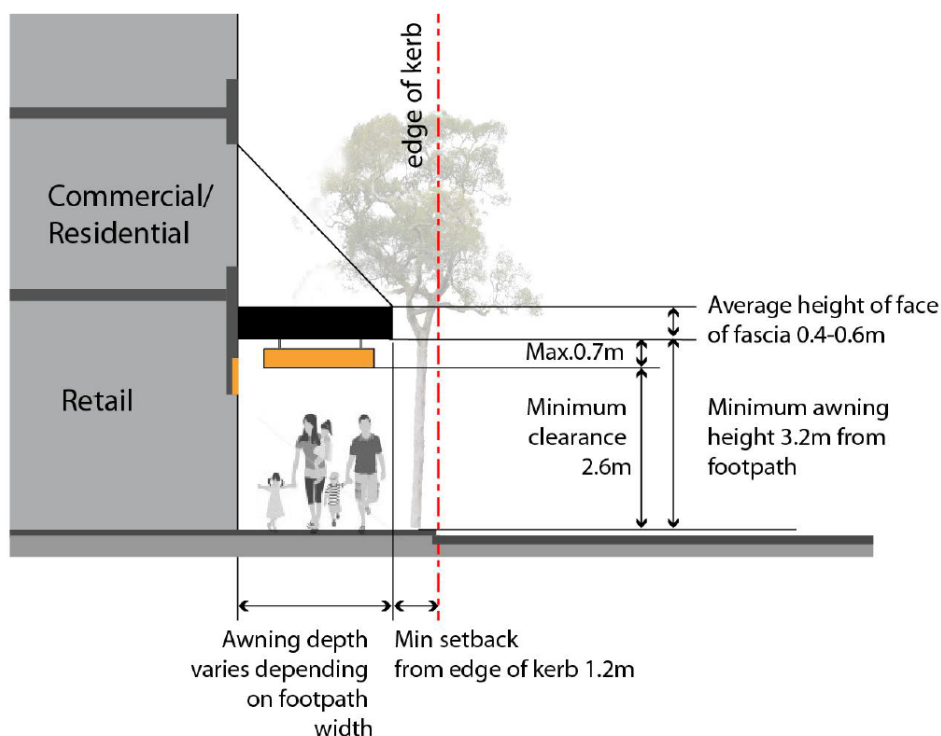
Figure 9. Awning Dimensions
