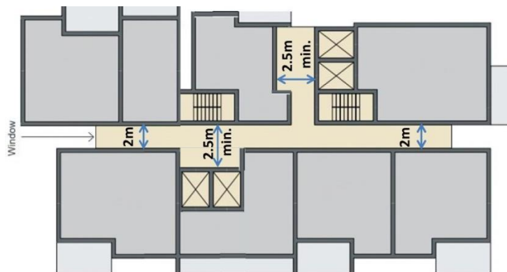
Figure 1(f): Corridor widths. (Adapted from ADG 2015)
