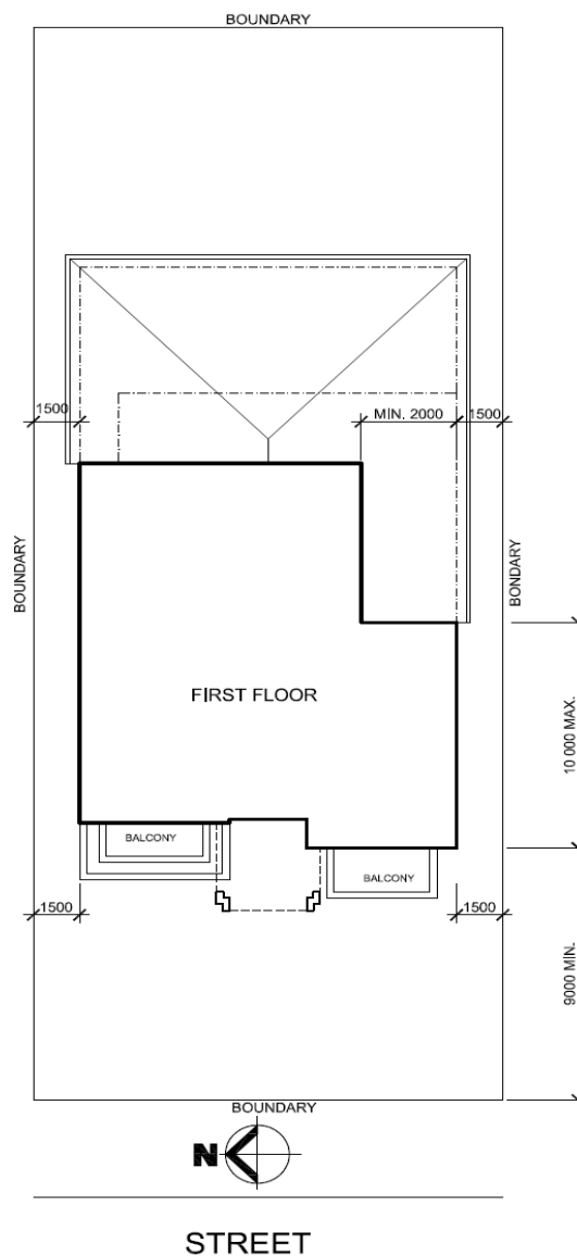
Figure 42: Setbacks to Minimise Overshadowing
