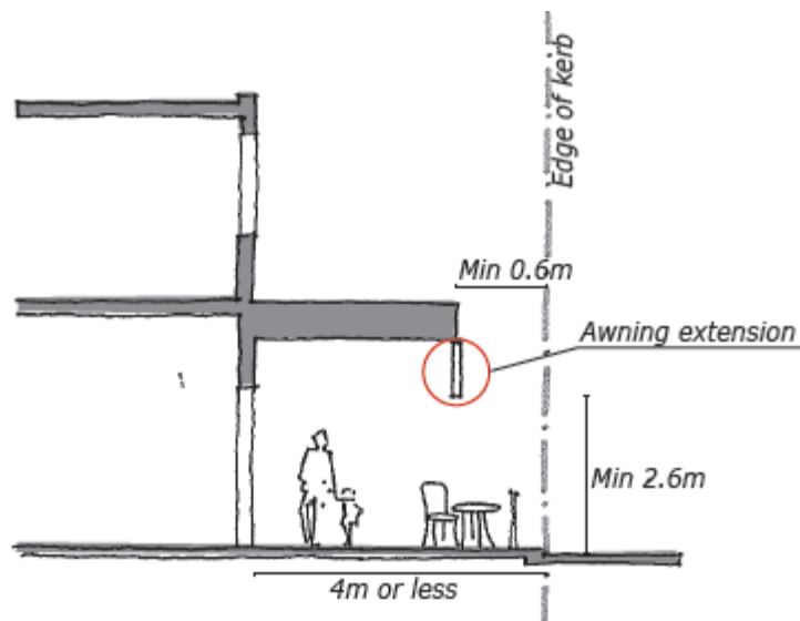
Figure 1(k): Straight Drop Awning Extensions
